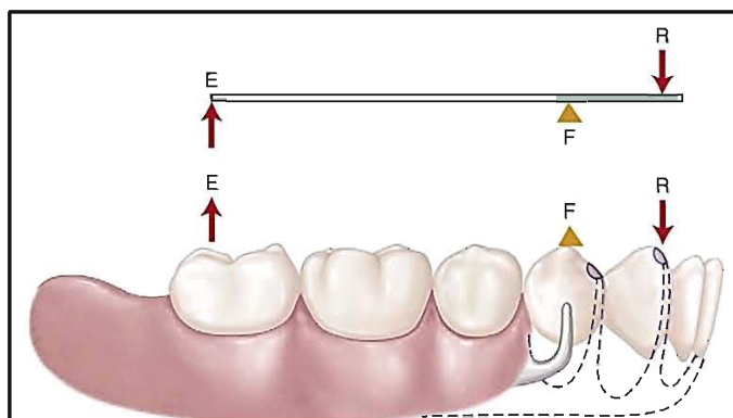
Figure 1: Action of the indirect retainer where E: Effort (e.g. sticky food), F: fulcrum line, & R: Resistance (indirect retention).
